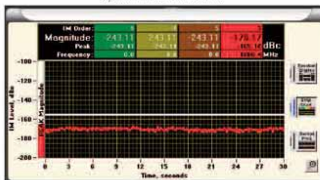
Dynamic PIM Test Results
